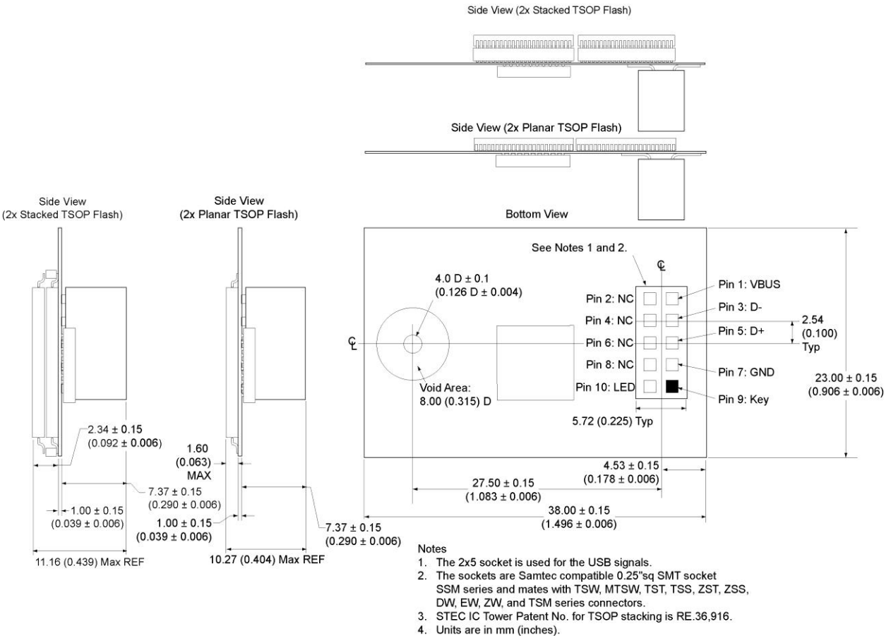
Figure 2: Mechanical Dimensions, Standard 2x5 Connector
